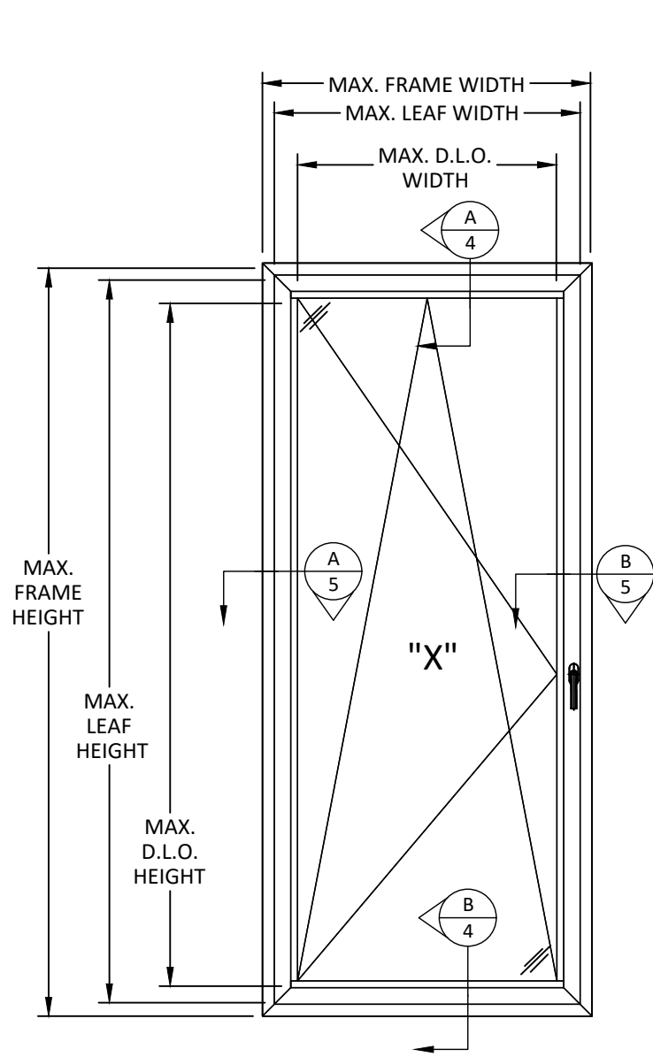
ELEVATIONS
