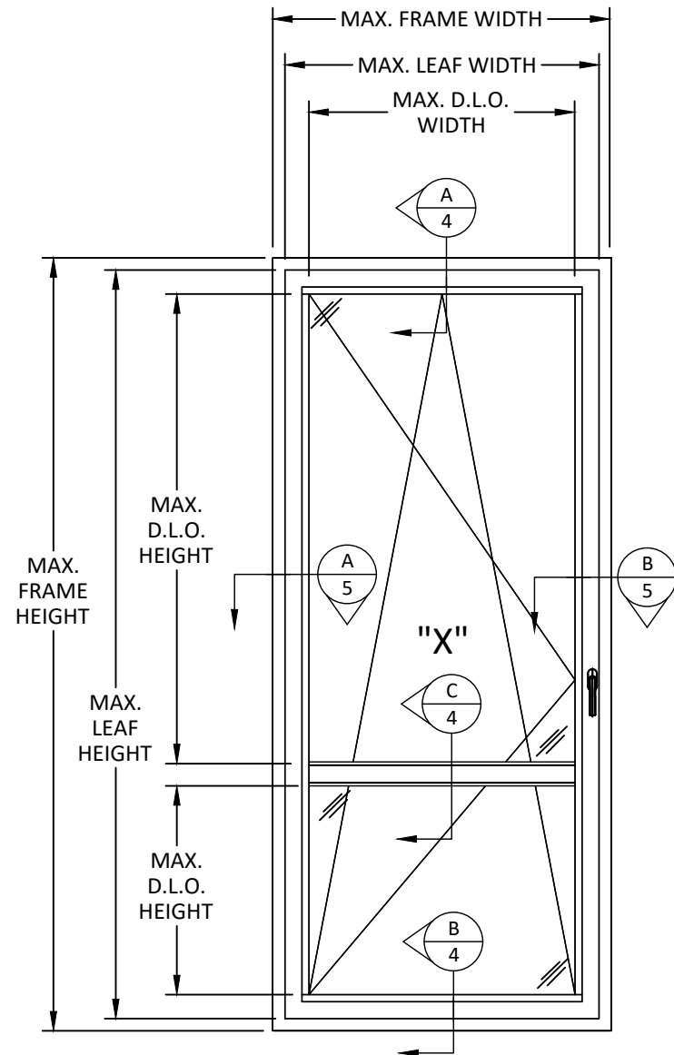
ELEVATIONS
